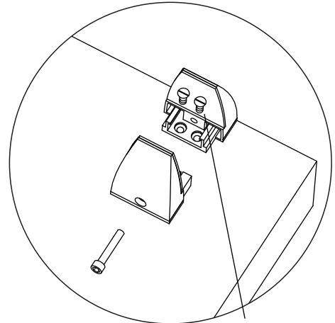
Use #6 Flathead Screw
